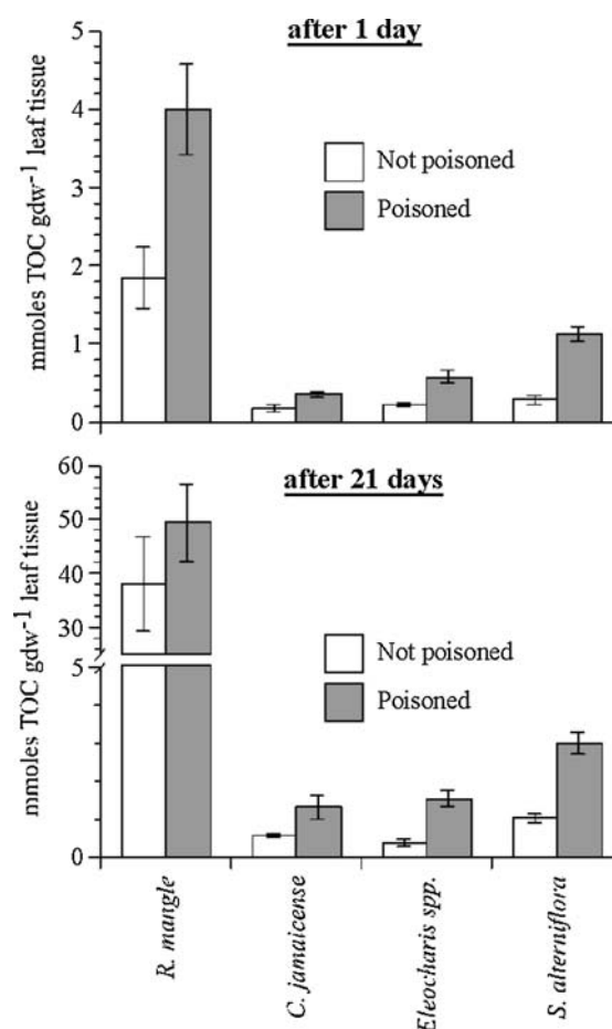
Figure 1. Releases of total organic carbon (TOC) from each of four species of leaf material with poison (gray bars) and without poison (white bars) incubated for 1 day (top graph) and for 21 days (bottom graph). Error bars represent standard deviations from three replicates. Axis break for bottom graph reveals the disparity in TOC release between R. mangle and three macrophyte species after 21 days of immersion in water.
