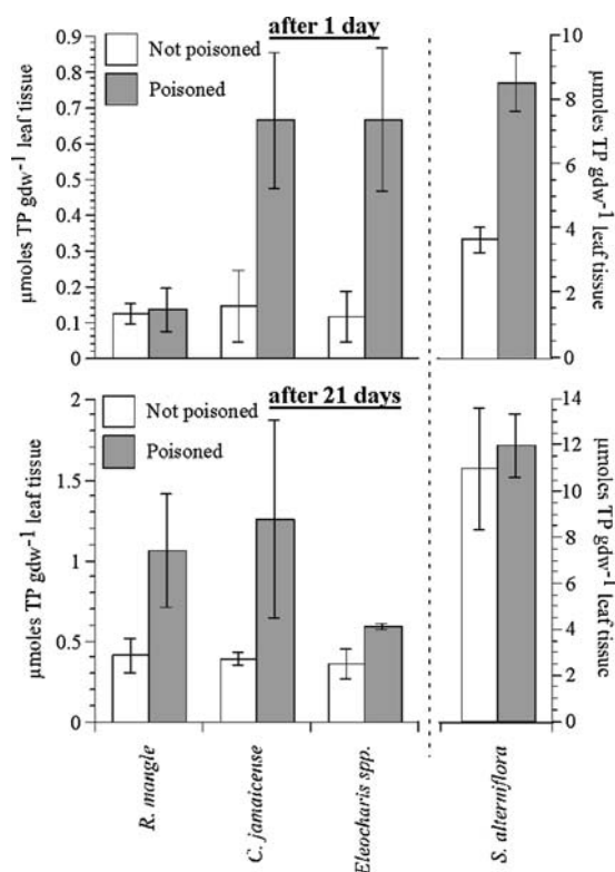
Figure 2. Releases of total phosphorus (TP) from each of four species of leaf material with poison (gray bars) and without poison (white bars) incubated for 1 day (top graph) and for 21 days (bottom graph). Error bars represent standard deviations from three replicates. Separate y-axis for S. alterniflora is intended to show the magnitude of TP released from a N-limited plant versus that of three P-limited, Everglades plant species after 1 and 21 days of immersion in water.
