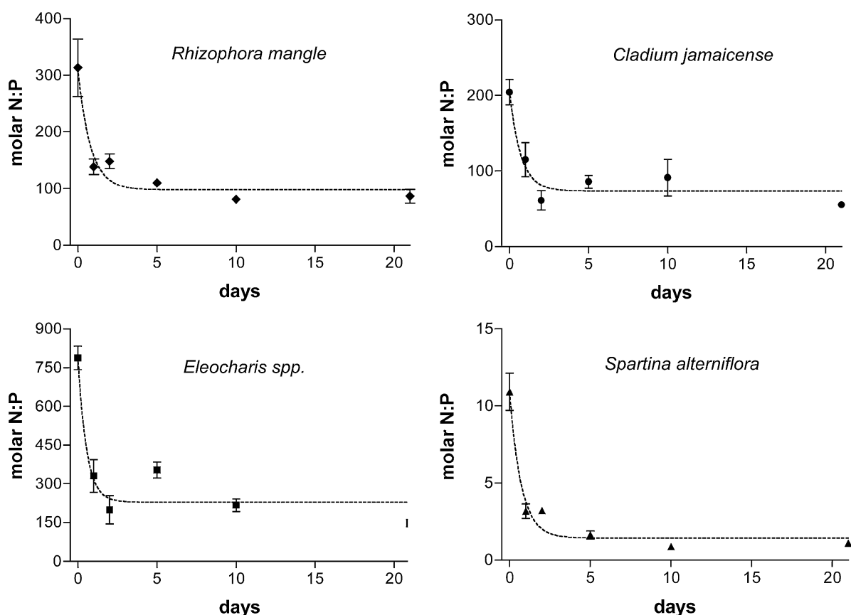
Figure 4. Scatter plot showing how TN:TP molar ratios in incubation water changed through time as a result of leaching and microbial activity associated with the early decay of all four macrophyte species. Data are from non-poisoned treatments only and error bars represent standard deviation of three replicates collected at each sampling interval.
