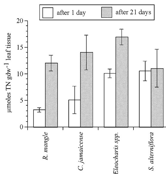
Figure 3. Releases of total nitrogen (TN) from each of four species of leaf material immersed in water without poison for 1 day (white bars) and 21 days (shaded bars). Error bars represent standard deviations from three replicates.
